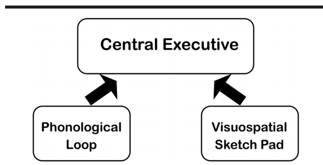
Figure 1. Schematic of the multicomponent model of working memory. More recently an episodic memory component has been added to the classic version of the model, but it is not relevant to this study.
