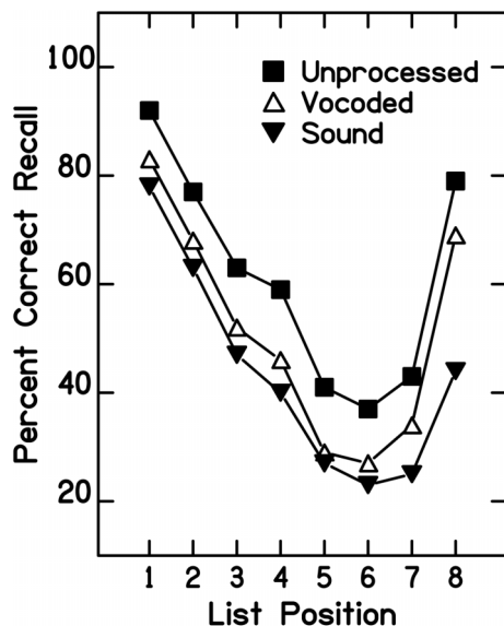
Figure 2. Classic U-shape function for serial recall of verbal material. Data replotted from Nittrouer and Lowenstein (2014), from adult subjects for unprocessed speech, eight-channel vocoded speech, and environmental sounds.
